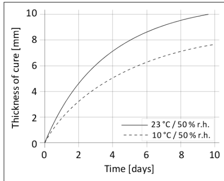
Diagram 1: Curing speed of Sikaflex®-502
